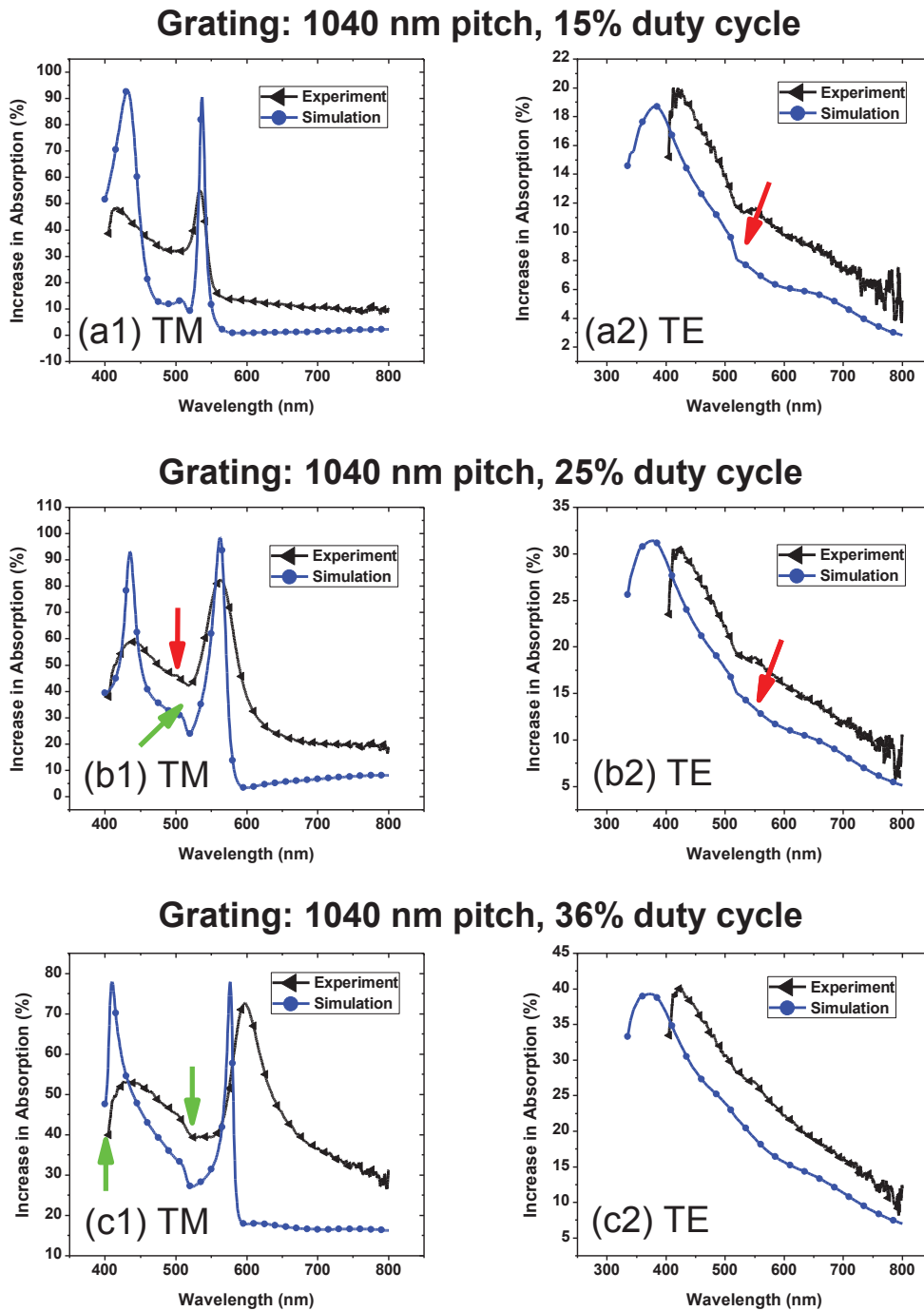
Fig. 5.4 Compared with a 100 nm flat Ag film, the absorption from bare Ag gratings is increased. The absorption peaks for different grating geometries are shown. The red arrows indicate the good agreement between COMSOL simulation and experimental results, while the green arrows mark the starting wavelengths of the SPP peaks.
