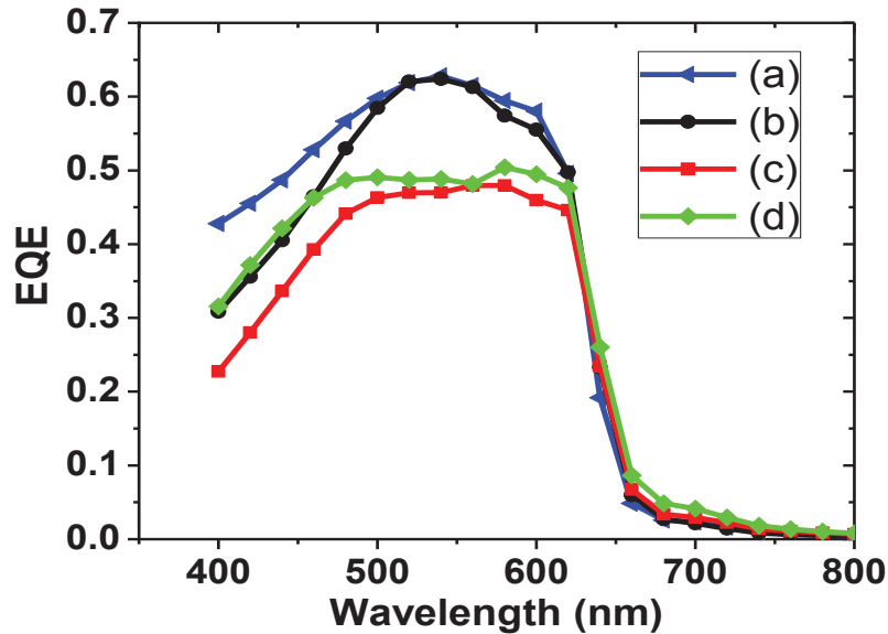
Fig. 6.7 EQE curves of the devices in Table 6.3. Device (a) is superstrate type with light incident from the bottom and Devices (b) ~ (d) are substrate type. Device (b) is the best substrate type device obtained, while device (c) and (d) suffered poor carrier collection in the absorption band of P3HT:PCBM.
