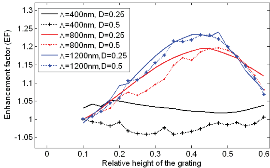
Fig. 3.5 Effect of the grating height on EF in J_{sc} for different combinations of \Lambda and D , which shows increase EF for larger grating height until it reaches the maxima and starts to decrease due to the reduced active layer.
