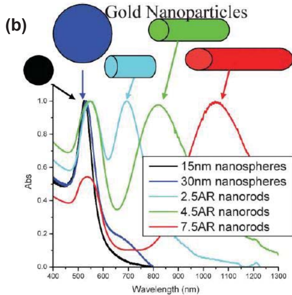
Fig. 2.3 (a) A true color, dark-field photograph of silver and gold nanoparticles of different sizes and shapes. Different colors suggest different resonance frequencies of the nanoparticles (from Ref. [22]). (b) When anisotropy is added to the gold nanoparticle, the growth of nanorods with higher aspect ratio (AR) in this case, the optical properties of the nanoparticles change more dramatically than those from the size change of the nanoparticles (from Ref. [28]).
