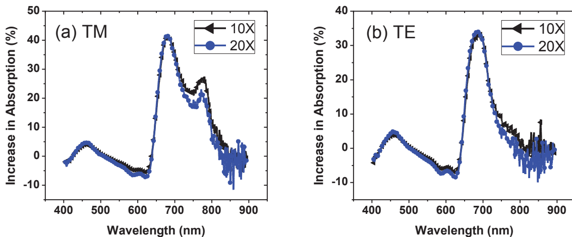
Fig. 4.11 Comparisons of light absorption enhancement results from OPVs with a grating on the bottom, for (a) TM waves and (b) TE waves. Objective lenses with different magnifications and thus different light acceptance angles are used.
