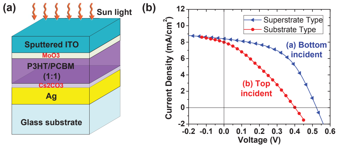
Fig. 6.6 (a) The substrate type inverted OPV on a planar Ag coated glass substrate. (b) JV curve of the best substrate type device ( \eta = 1.11\% ) is plotted (red curve). A 120 nm ITO and a 15 nm MoO 3 consist the anode, a 2 nm thermally evaporated Cs 2 CO 3 layer and a 100 nm Ag layer consist the cathode. For comparisons, the JV characteristic of the superstrate type device with light incident from the bottom is also superposed (the blue line).
