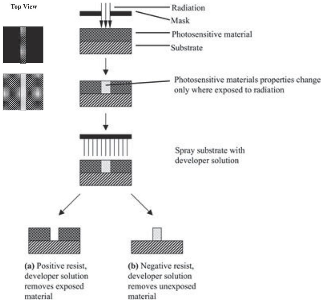
Fig. 4.1 Different pattern definitions in (a) a positive photoresist and (b) a negative photoresist transferred from the same original pattern, which is a shadow mask in this example. (from Ref. [83])
